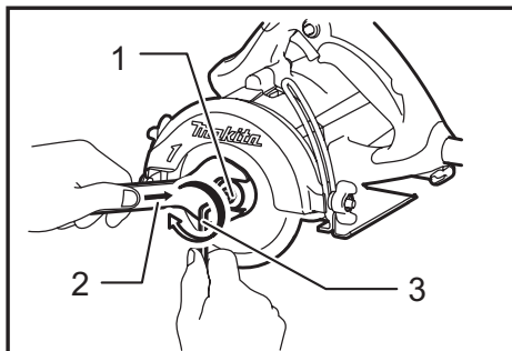
► 1. Outer flange 2. Wrench 3. Hex wrench
